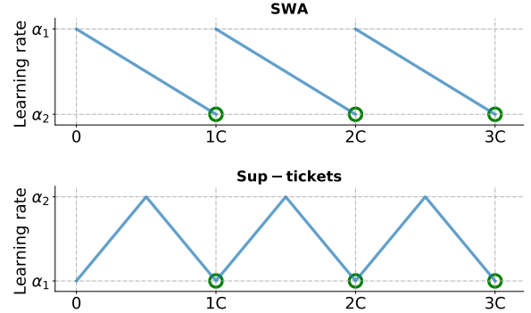
Figure 2: Top: cyclical learning rate schedule of Garipov et al. [2018]. Bottom: cyclical learning rate schedule of Sup-tickets. Cheap tickets are collected at the end of each learning rate schedule cycle (green circles in the figure).
